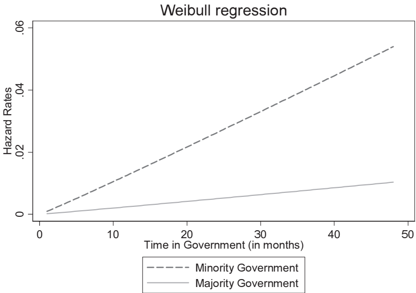
Figure 2 Underlying Hazard Rates for Majority and Minority Governments (Model 1)
