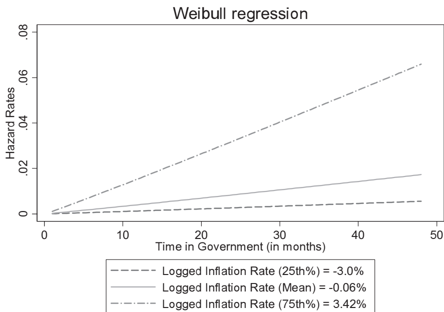
Figure 3 Underlying Hazard Rates for Varying Inflation Rates (Model 1)
