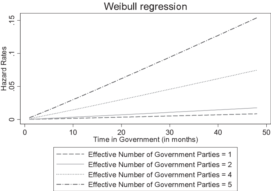
Figure 1 Underlying Hazard Rates for Number of Government Parties (Model 1)
